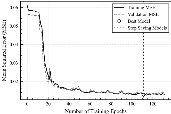
Learning Curve of LSTM Model for SolarPlant-1 (Gyeongju)
